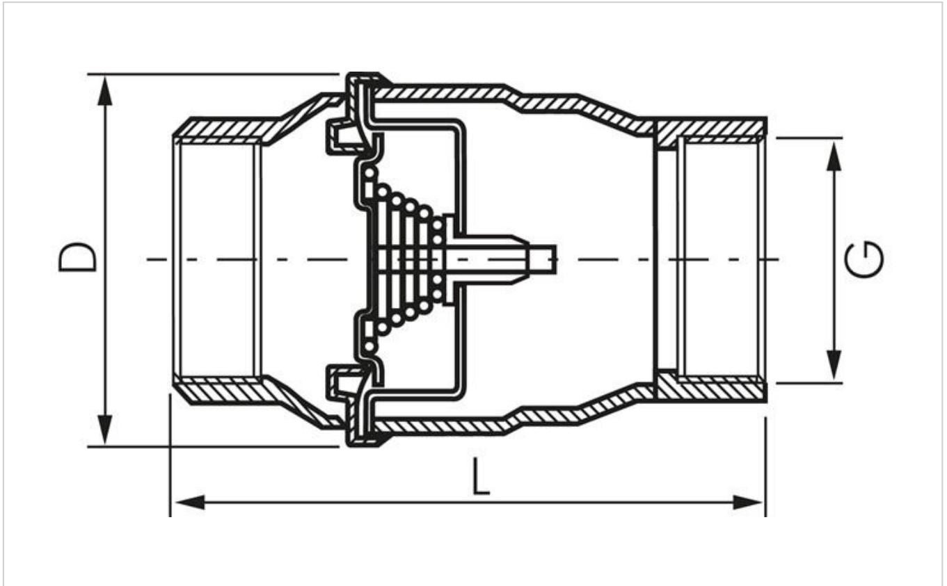
Drawing: Check valve
